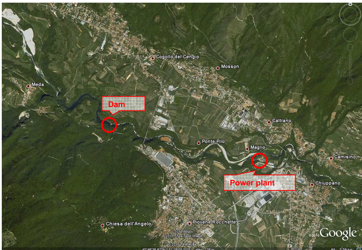
Figure 1: Aerial view of the Astico reach concerned by the Bessé power plant
