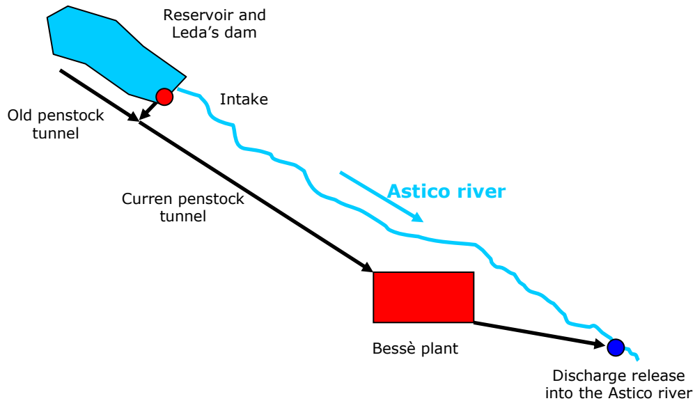
Figure 5: Power plant scheme.
